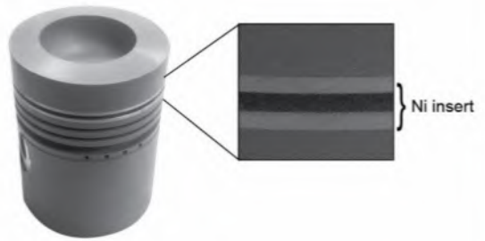
AlfinGold Piston
